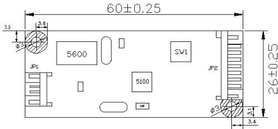
PenMount 5126BH Control Board
